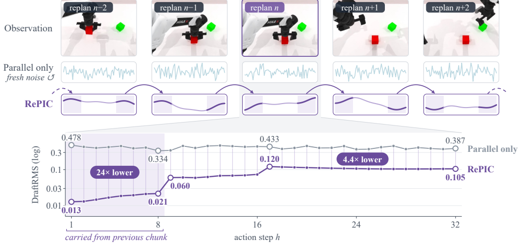
Figure 4: Trajectory reuse lowers draft error. Top : five consecutive RoboTwin 2.0 replans; RePIC carries each unexecuted suffix into the next chunk (shaded), whereas Parallel only starts from a linear draft of fresh noise. Bottom : DraftRMS per action step h (log scale), fixed R = 24 .
