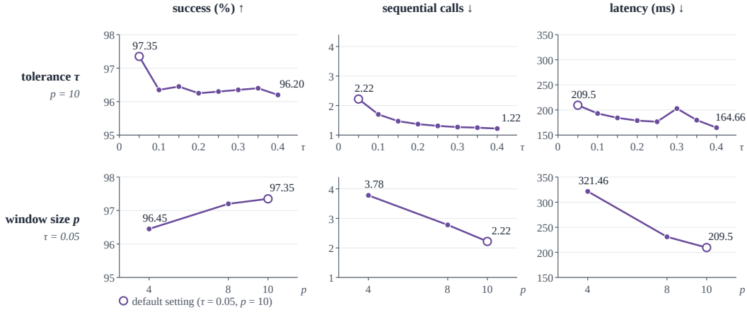
Figure 7: Sensitivity to the tolerance and the window size. Fast-WAM on LIBERO (average over the four suites), one hyperparameter varied at a time from the default setting (open marker; \tau=0.05, p=10 ). Top : stride tolerance \tau at p=10 . Bottom : window size p at \tau=0.05 . Calls and latency are per chunk. The default setting is the RePIC row of Tab. 3; latencies were re-timed within the sweep.
