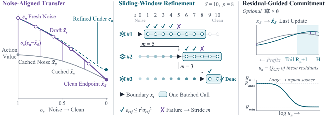
Figure 3: Mechanisms of RePIC. Left: noise alignment of one action position. Middle: a warm-started solve finishes in three batched calls (shaded: updated states). Right: residual-guided commitment maps tail residuals to the next execution length R_{n+1} .
