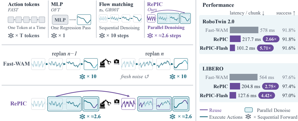
Figure 1: Don’t throw away the solution. Left: RePIC combines trajectory reuse with parallel denoising, reducing sequential velocity network calls from 10 to 2.2–2.6 per chunk on Fast-WAM. Right: action-generation latency and task success of Fast-WAM and its RePIC variants on RoboTwin 2.0 and LIBERO. Latency excludes action execution and simulator stepping.
