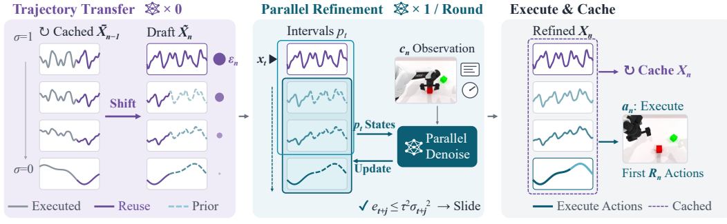
Figure 2: One replan of RePIC. Curves are action chunks, from noisy to clean states. Left: shift, fill, and align the cached trajectory to fresh noise without network calls. Middle: refine under c_n with one batched network call per round. Right: execute the R_n -action prefix and cache the trajectory.
